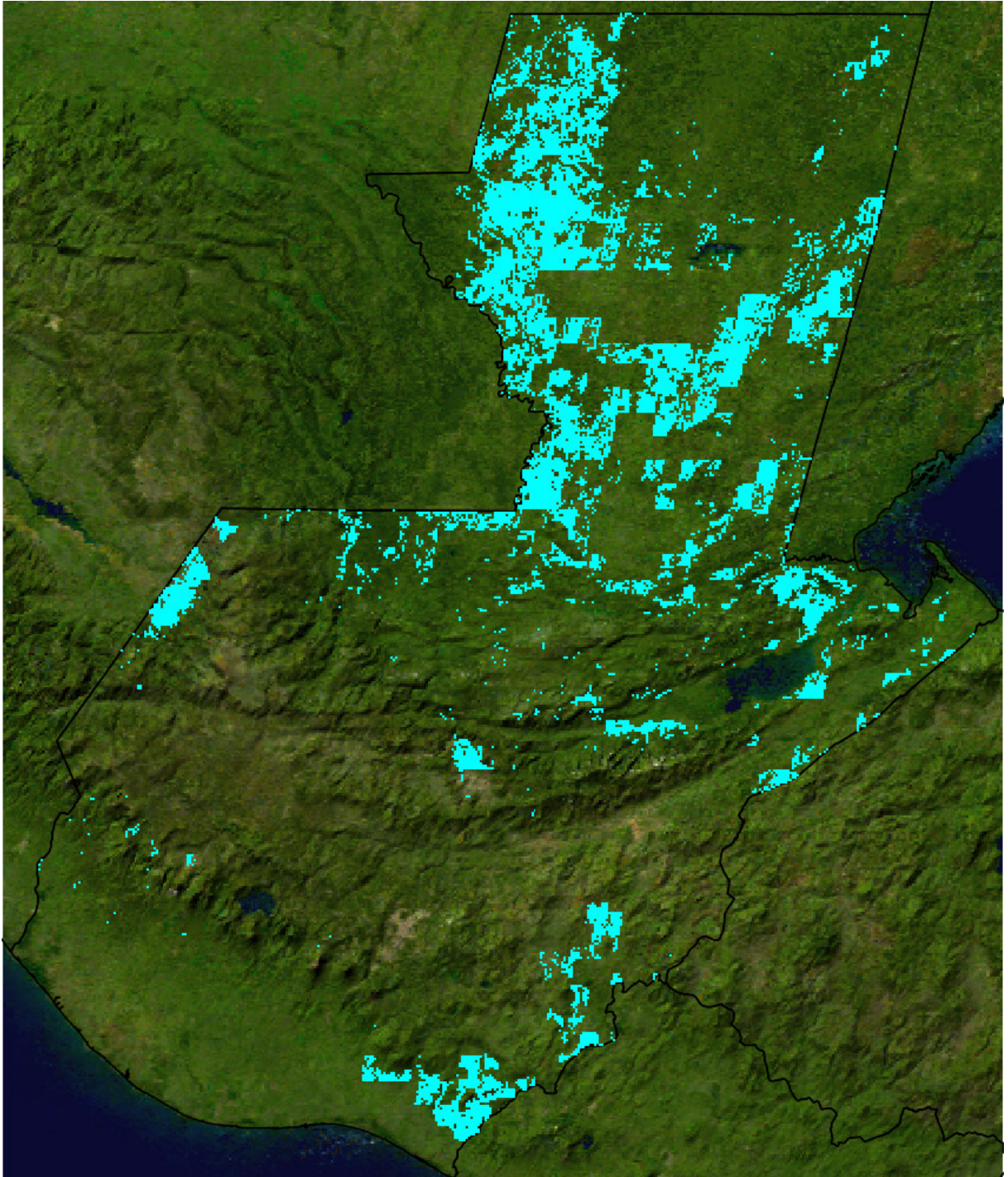
Figure 14: Restoration of 40% of deforested lands. Priority locations for restoration (cyan) for a solution that represents a balance between climate change mitigation and biodiversity conservation objectives while maximising cost-effectiveness (benefit/cost).
