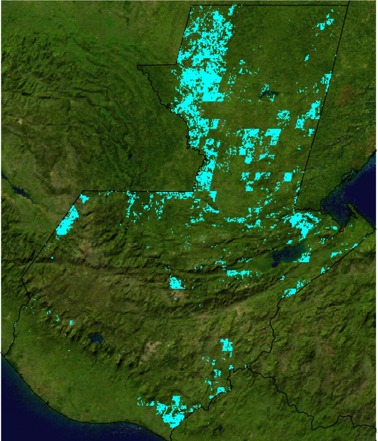
Figure 11: Restoration of 30% of deforested lands. Priority locations for restoration (cyan) for a solution that represents a balance between climate change mitigation and biodiversity conservation objectives while maximising cost-effectiveness (benefit/cost).
