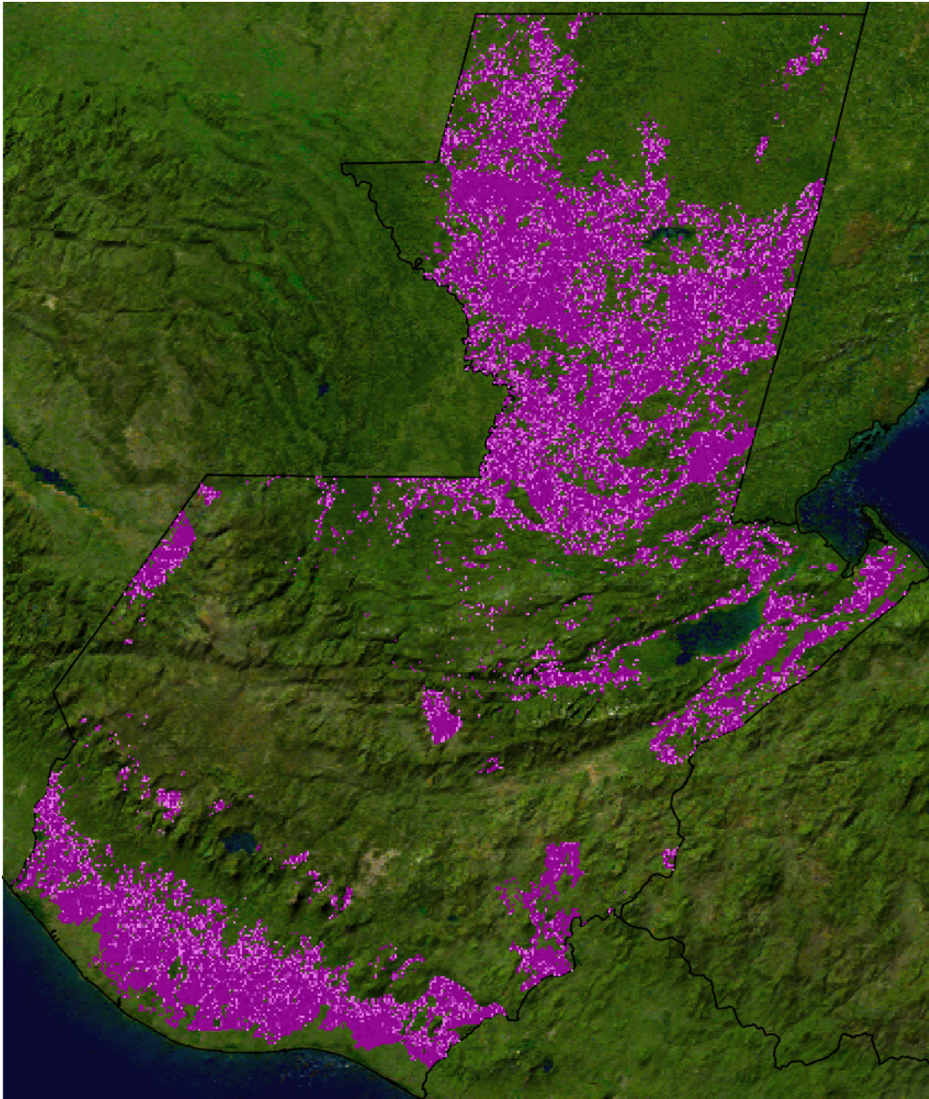
Figure 2: Area deemed available for forest restoration. Areas in purple indicate the 1 km 2 planning units that were assessed to have potential for forest restoration given (see Methods for details). The shading of cells from light to dark purple is proportional to the area within each planning unit available for forest restoration.
