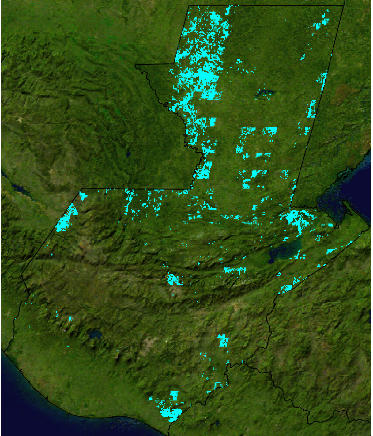
Figure 8: Restoration of 20% of deforested lands. Priority locations for restoration (cyan) for a solution that represents a balance between climate change mitigation and biodiversity conservation objectives while maximising cost-effectiveness (benefit/cost).
