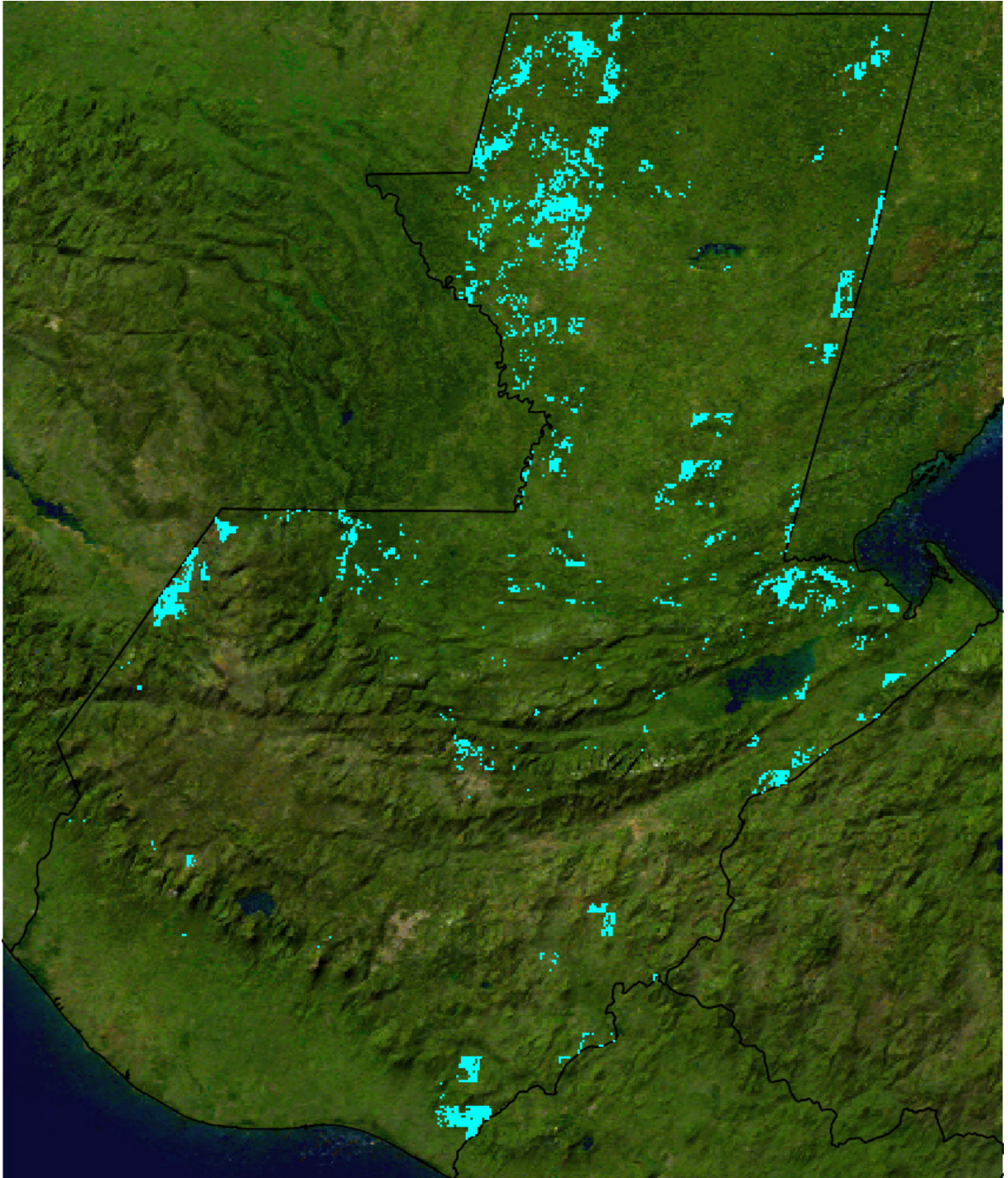
Figure 5: Restoration of 10% of deforested lands. Priority locations for restoration (cyan) for a solution that represents a balance between climate change mitigation and biodiversity conservation objectives while maximising cost-effectiveness (benefit/cost).
