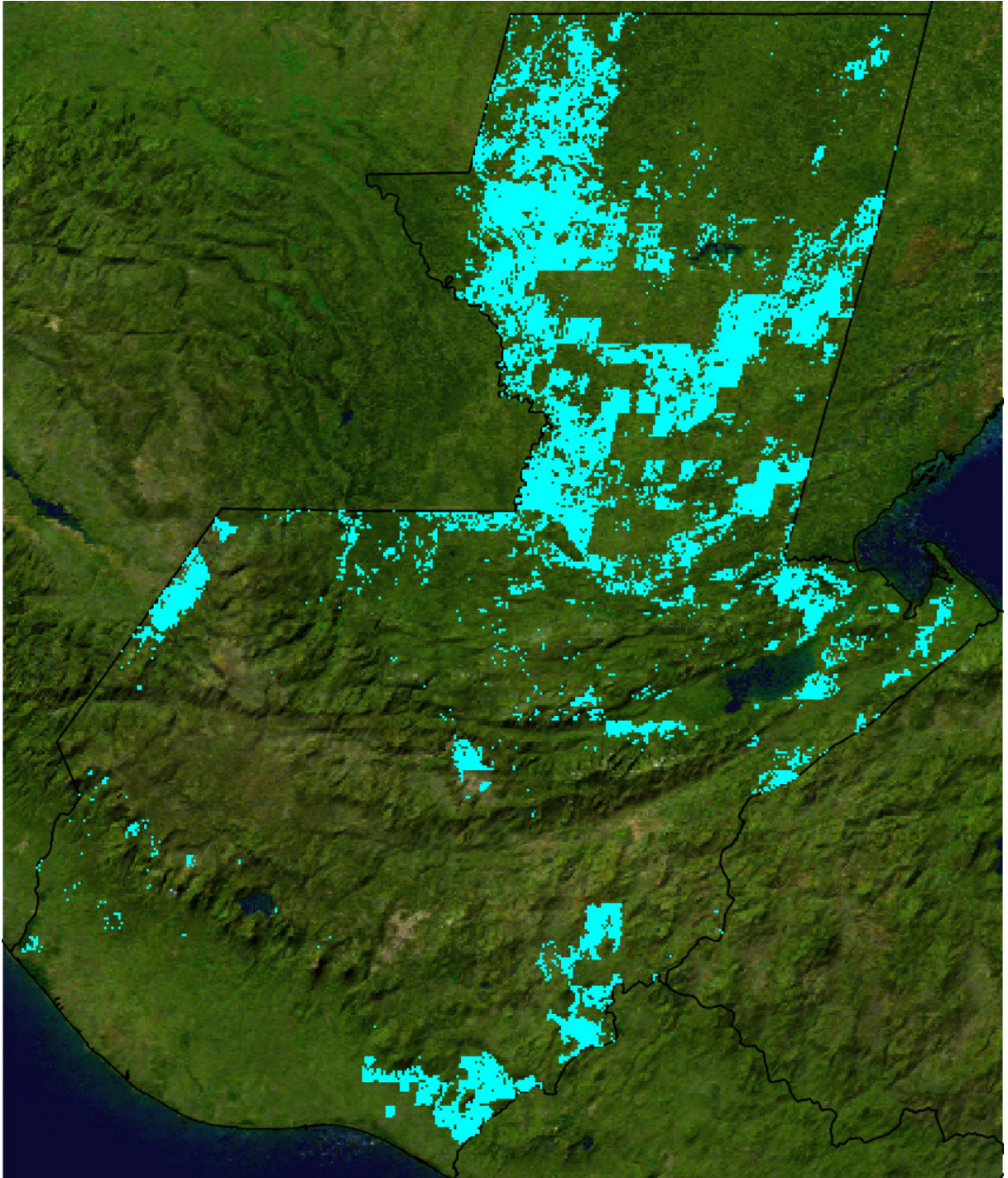
Figure 17: Restoration of 50% of deforested lands. Priority locations for restoration (cyan) for a solution that represents a balance between climate change mitigation and biodiversity conservation objectives while maximising cost-effectiveness (benefit/cost).
